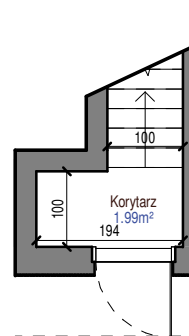
PARTER
